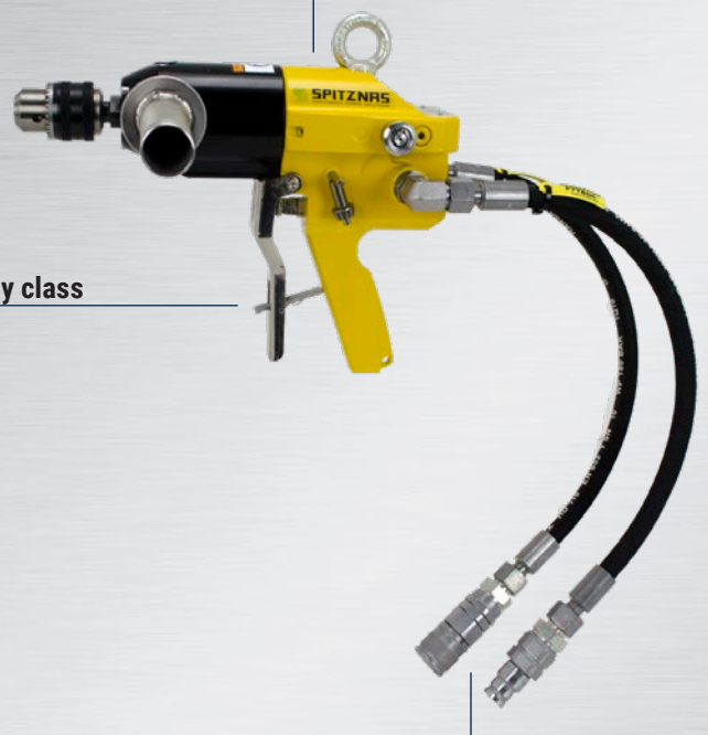
Hydraulic hose set
