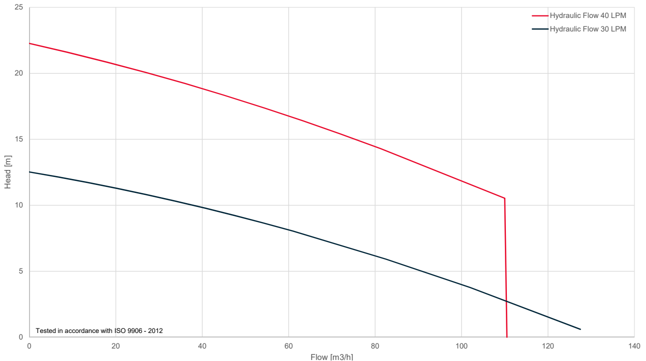
4" Submersible Pump
