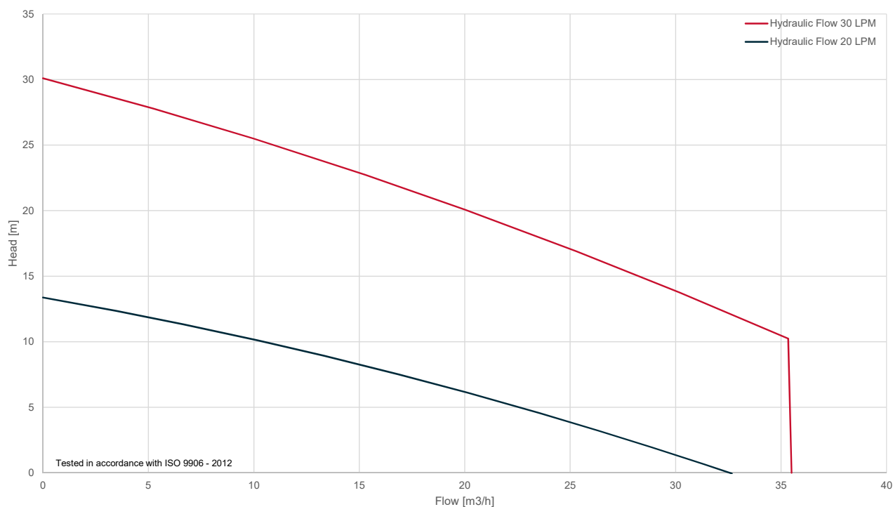
2" Submersible Pump
