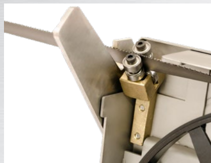
Saw blade guide
