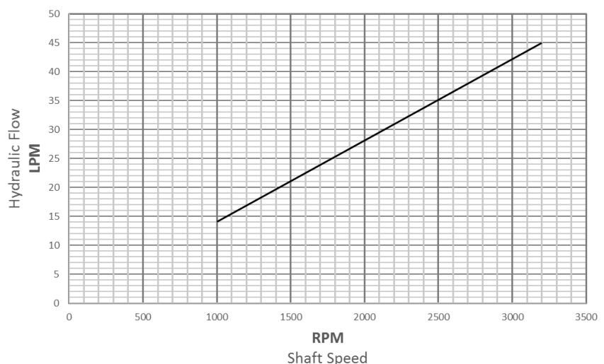
GR29 Hydraulic Flow Vs Shaft Speed
